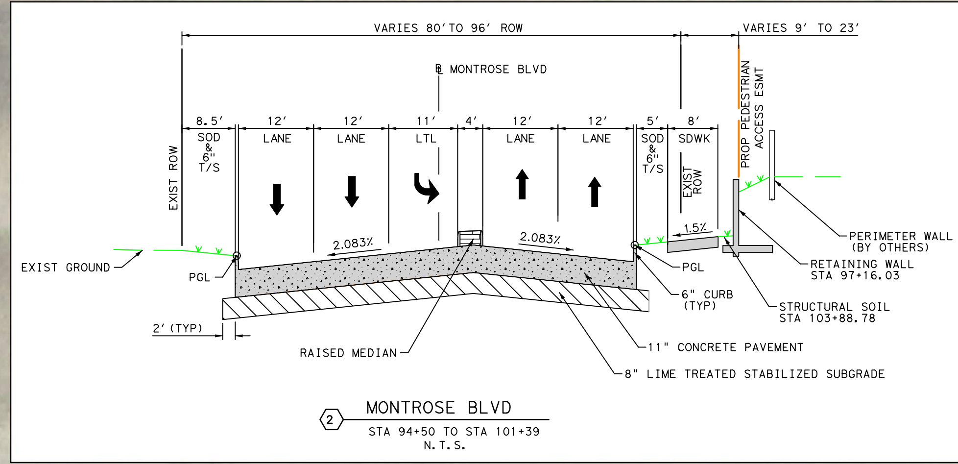
PROPOSED TYPICAL SECTION WITH SB LEFT TURN LANE
