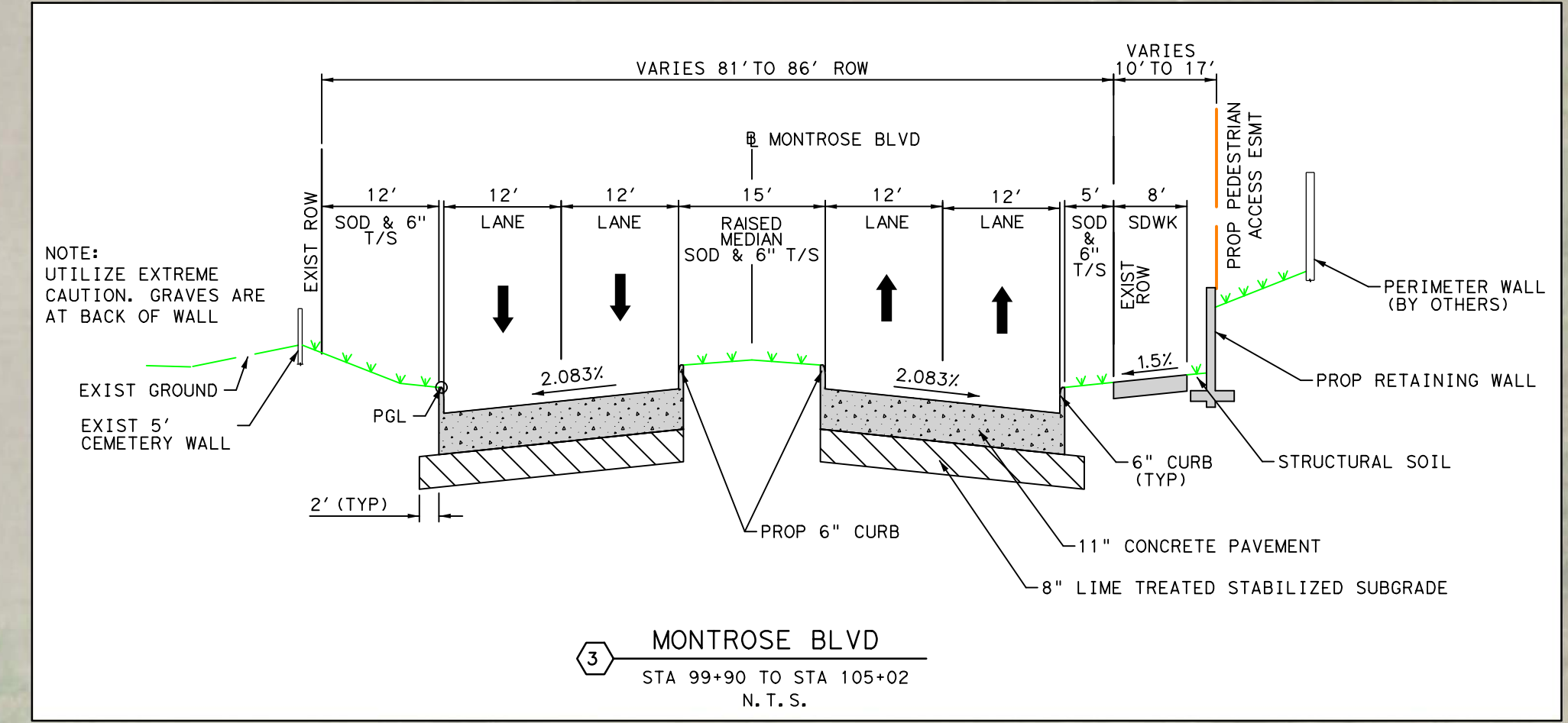
PROPOSED TYPICAL SECTION NORTH OF ISMAILI CENTER TO ALLEN PKWY
