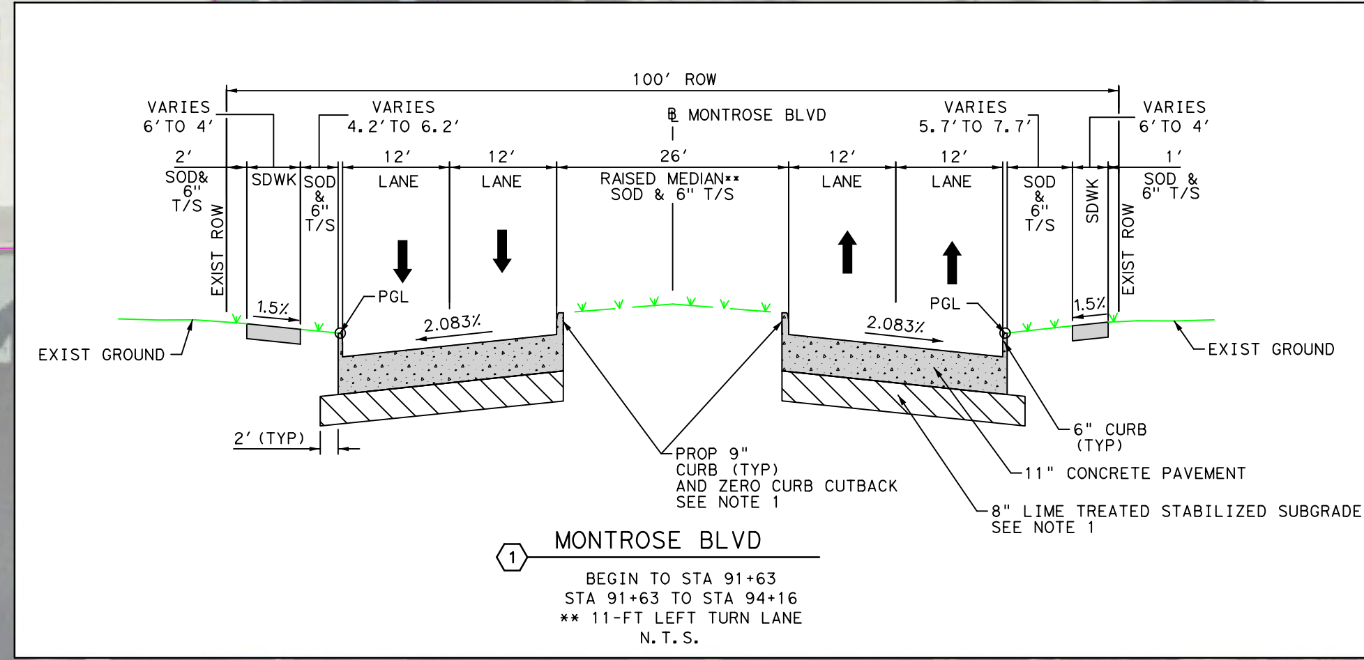
PROPOSED TYPICAL SECTION FROM W. CLAY ST. TO W. DALLAS ST.
